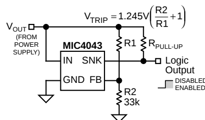
Figure 1. Voltage Detector
