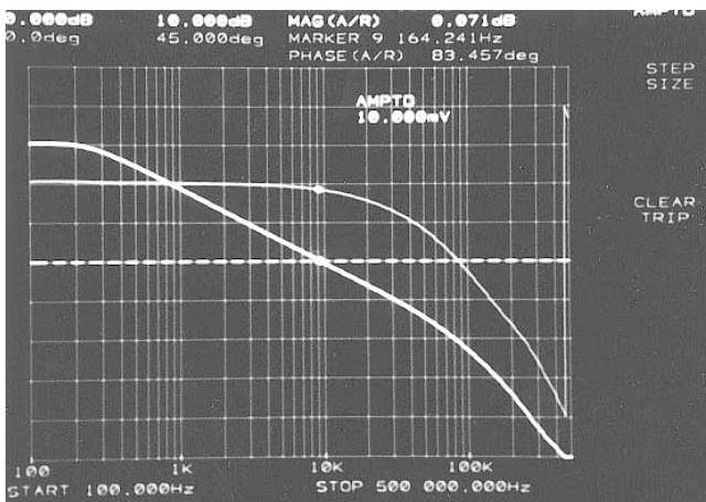
Figure 4a. 2.5V/1A Bode Plot ( \theta margin = 83^\circ )
