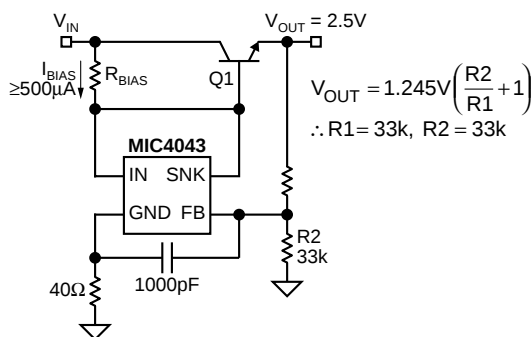
Figure 2. High-Current Regulator
