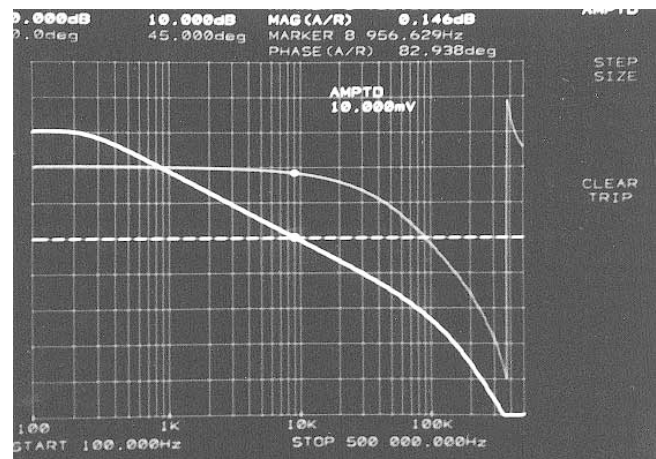
Figure 4b. 2.5V/2A Bode Plot ( \theta margin = 83^\circ )
